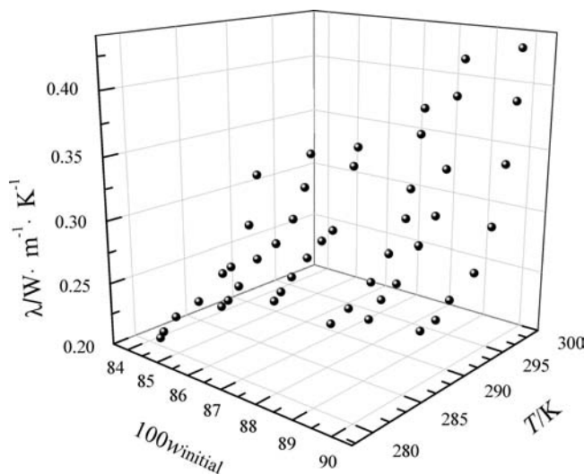
Figure 8. Thermal conductivity \lambda vs temperature T from (280.15 to 298.15) K and mass fraction w from (84.2 to 90.0) %.
