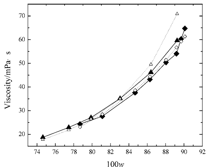
Figure 5. Viscosity data (298.15 K) comparison with literature 3 and eq 14. Data in this paper: \blacklozenge , measured data; \diamond , data calculated by eq 12. Data in literature 3: \blacktriangle , measured data; \triangle , data calculated by eq 14.
