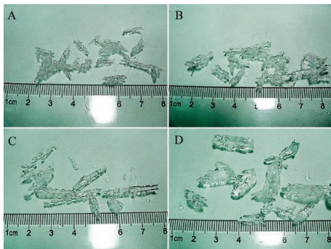
Figure 9. \text{H}_3\text{PO}_4 \cdot 0.5\text{H}_2\text{O} crystal with different initial mass fractions w_{\text{initial}} : A, 85.5 %, 282.65 K; B, 86.8 %, 283.7 K; C, 88.7 %, 286.85 K; D, 90.0 %, 286.85 K.
