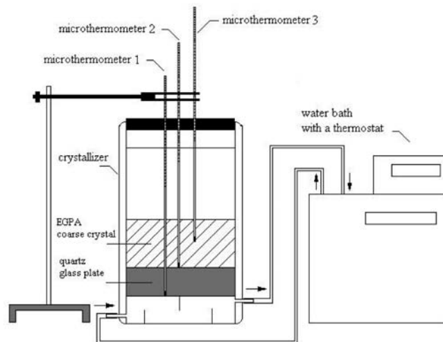
Figure 1. Schematic diagram of the experimental apparatus for measuring the thermal conductivity of EGPA coarse crystal.
