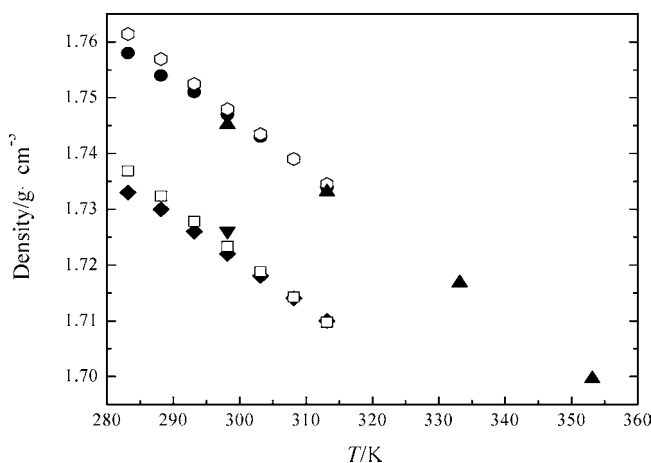
Figure 4. Density data comparison with literature. 2 Data in this paper: \blacklozenge , 88.0 %, (283.15 to 313.15) K; \bullet , 90.1 %, (283.15 to 313.15) K. Data calculated by eq 13: \square , 88.0 %, (283.15 to 313.15) K; \circ , 90.1 %, (283.15 to 313.15) K. Data in literature 2: \blacktriangledown , 88.28 %, 298.15 K; \blacktriangle , 90 %, (298.15 to 353.15) K.
