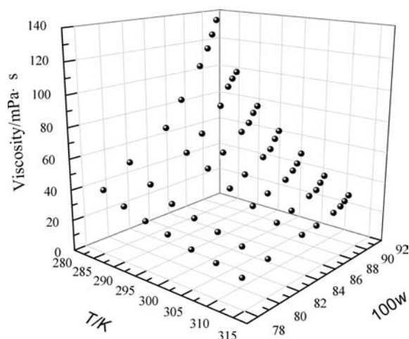
Figure 2. Viscosity \eta vs temperature T from (283.15 to 313.15) K and mass fraction w from (78.5 to 90.5) %.
