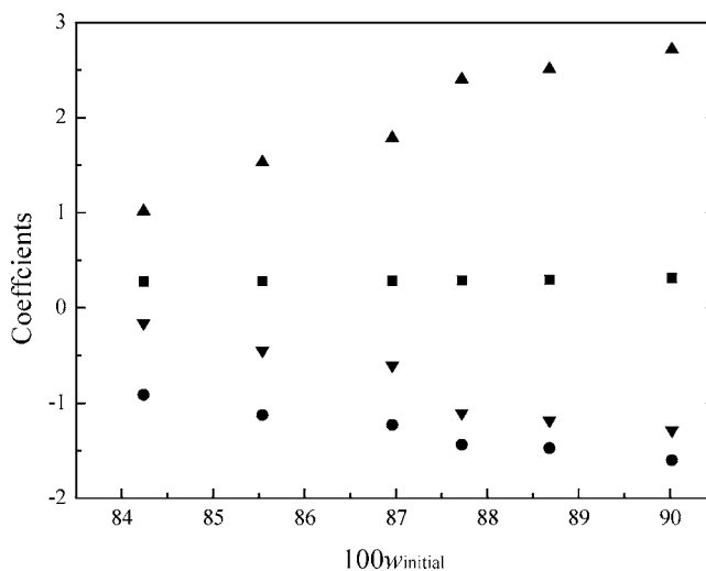
Figure 7. Coefficients A_0 , A_1 , A_2 , and A_3 in eq 15 vs initial mass fraction w from (84 to 90) %. \nabla , A_0 ; \blacktriangle , 10A_1 ; \blacksquare , 100A_2 ; \bullet , 1000A_3 .
